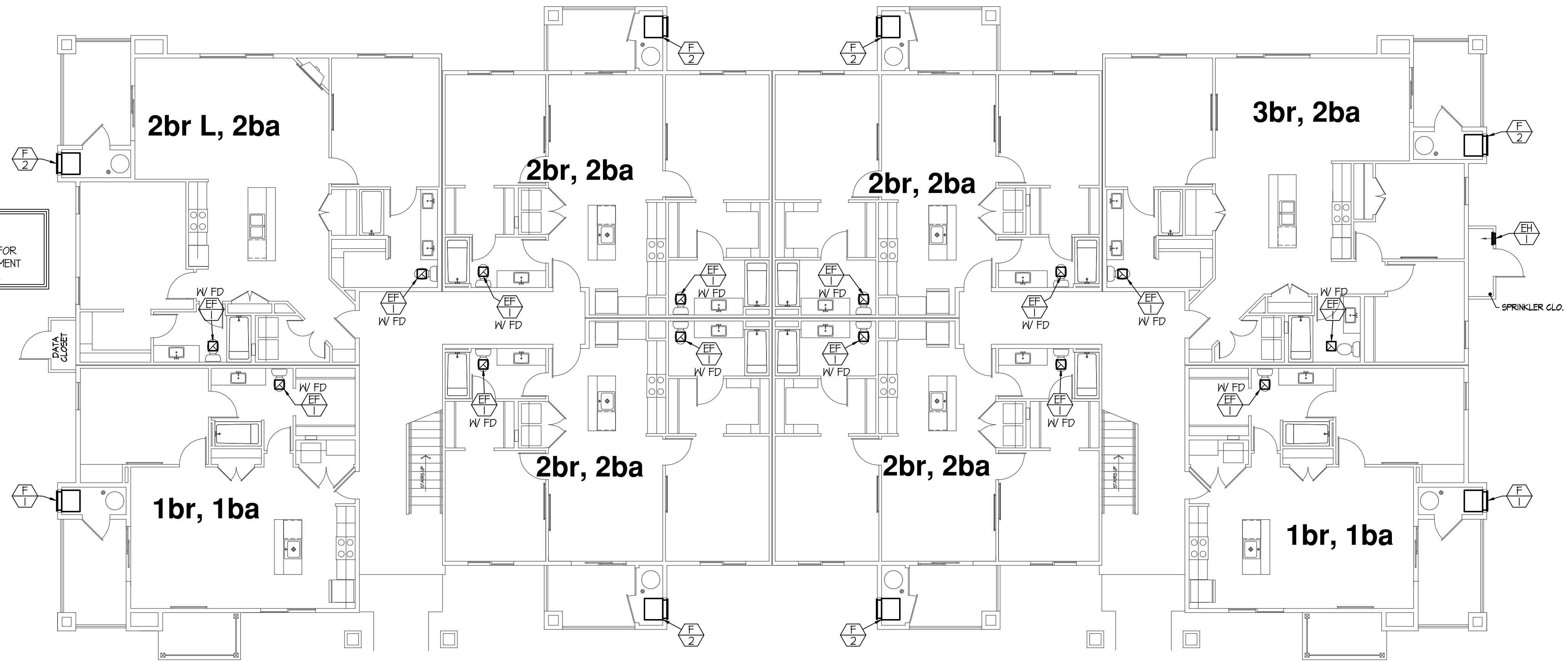
1ST FLOOR MECHANICAL PLAN SCALE: 1/8" = 1'-0"
