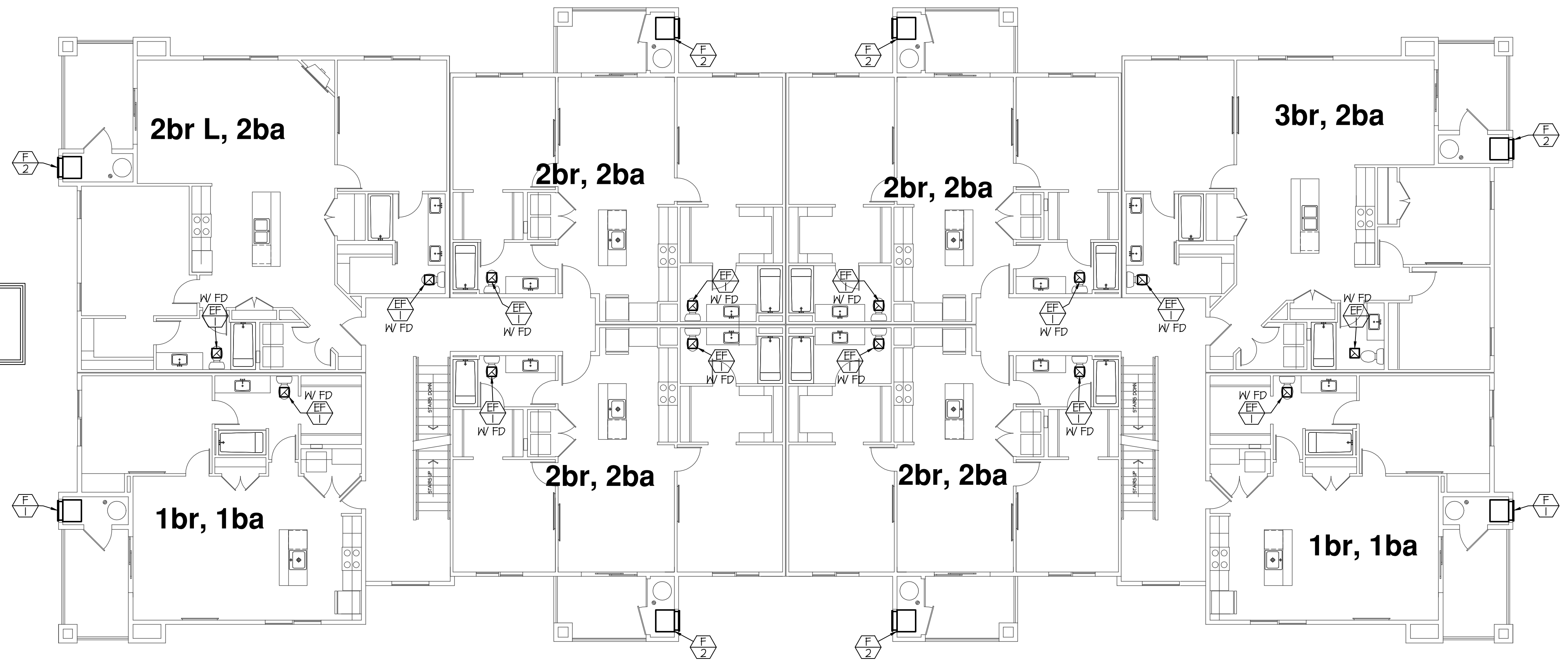
2ND FLOOR MECHANICAL PLAN SCALE: 1/8" = 1'-0"
